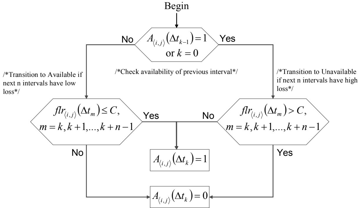
Figure 10 – Flowchart Definition of A_{i,j}(\Delta t_k)
