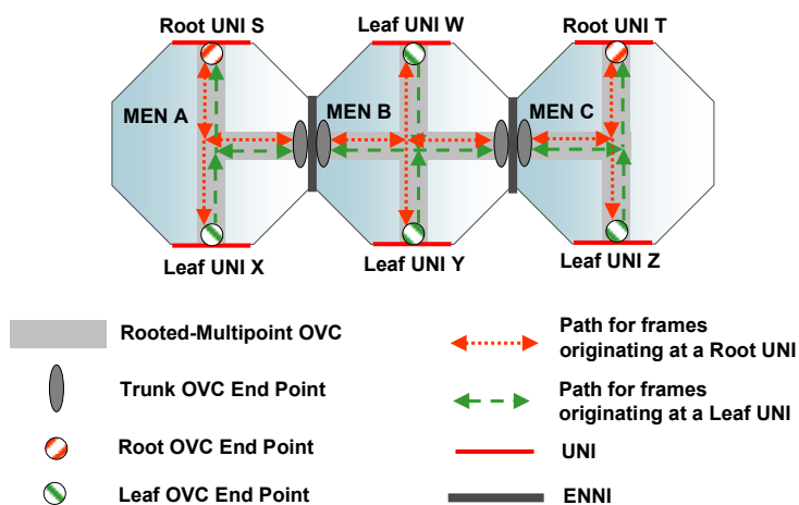
Figure 30 – Rooted-Multipoint EVC using Trunk OVC End Points
