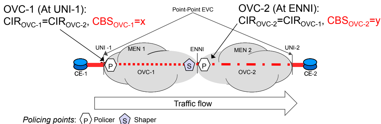
Figure 7 – Burst Alignment Example with Policing Points for Traffic Traversing the ENNI
