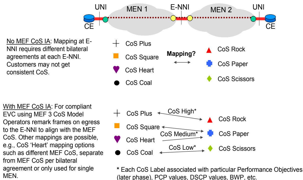
Figure 2 – CoS IA Motivation Example – E-NNI Mapping
